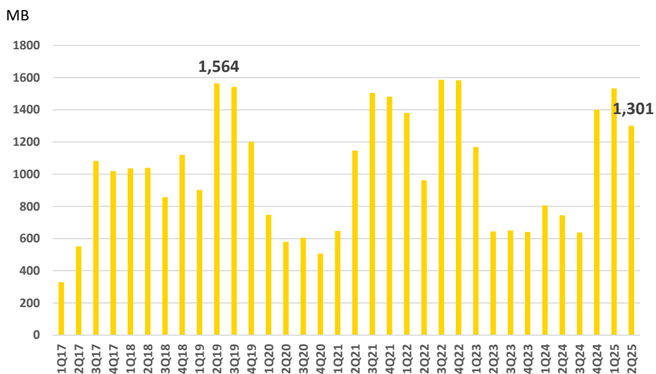
Fig. 1: PYLON Backlog
