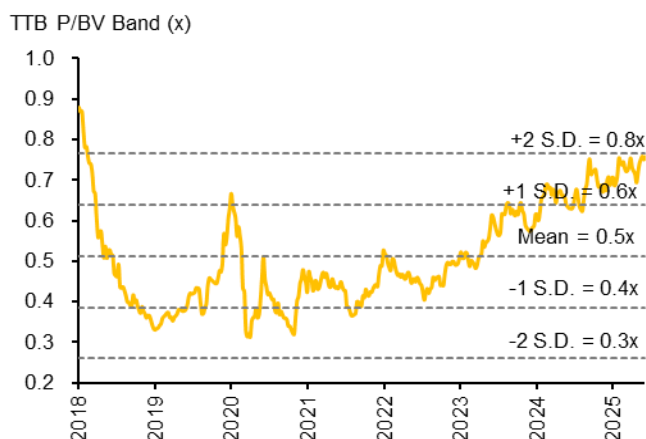
Fig. 2: Forward PBV band – TTB
