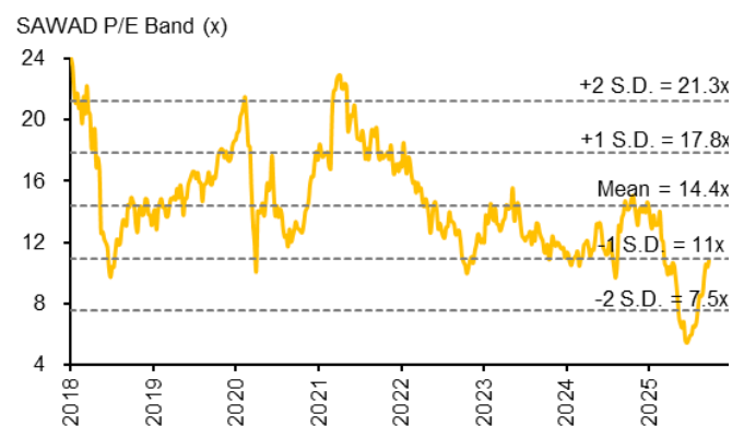
Fig. 3: Forward PER band – SAWAD
