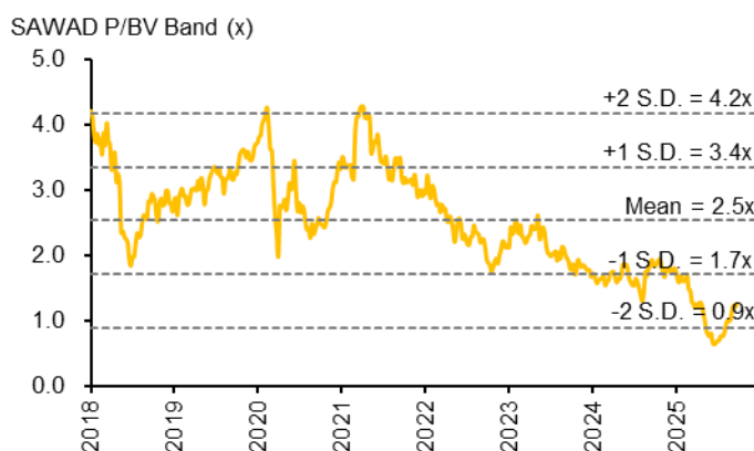
Fig. 2: Forward PBV band – SAWAD
