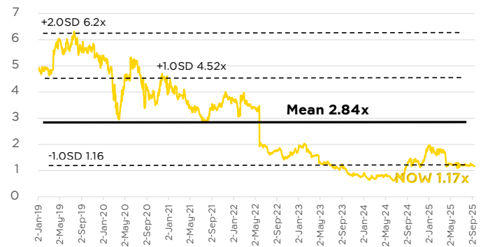
Fig. 3: Trailing P/BV band
