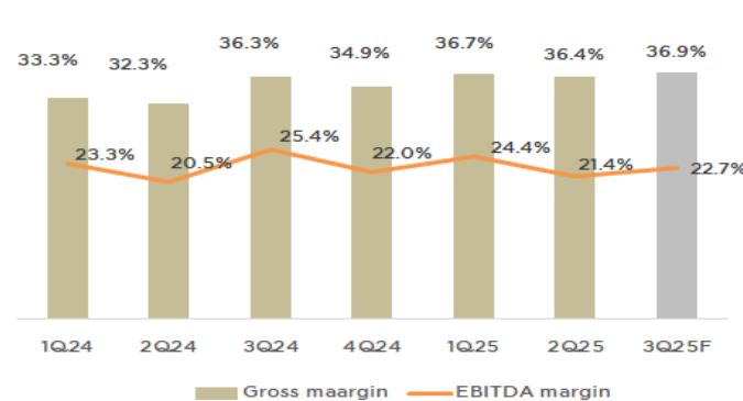
Fig. 3: PR9's Profitability
