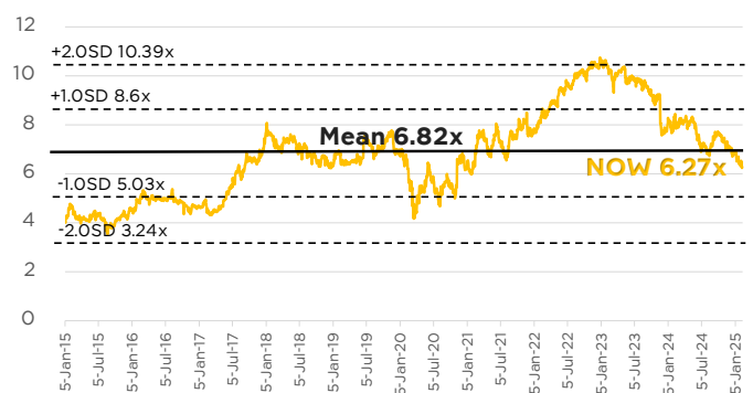
Fig. 5: AOT's Trailing PBV
