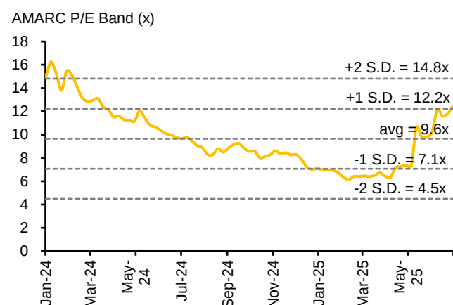
Fig. 9: AMARC's Prospective P/E band
