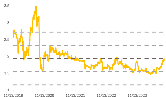
Fig. 4: Forward P/BV band
