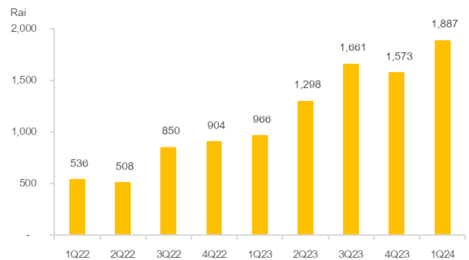
Figure 5: Accelerating backlog
