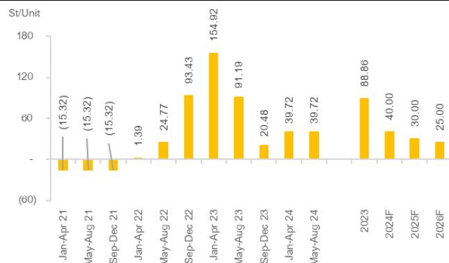
Figure 7: Ft rate
