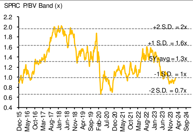
Figure 2: Prospective P/BV Band
