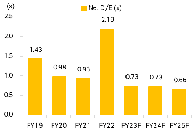
Figure 5: Net D/E dropped in FY23 given IPO proceeds
