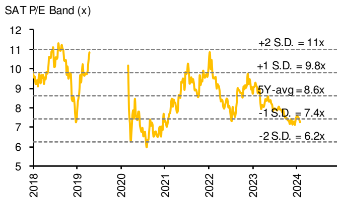
Figure 2: P/E band
