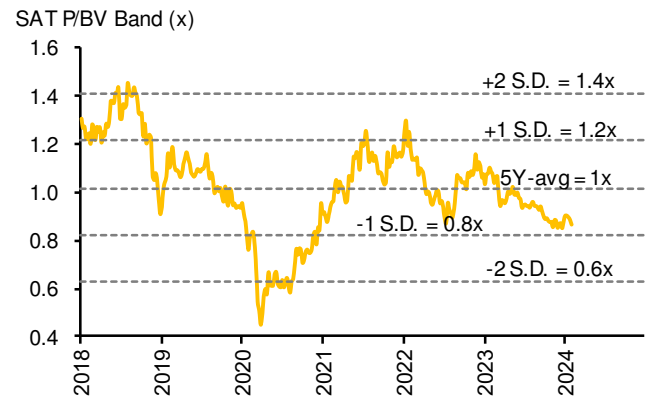
Figure 3: P/BV band
