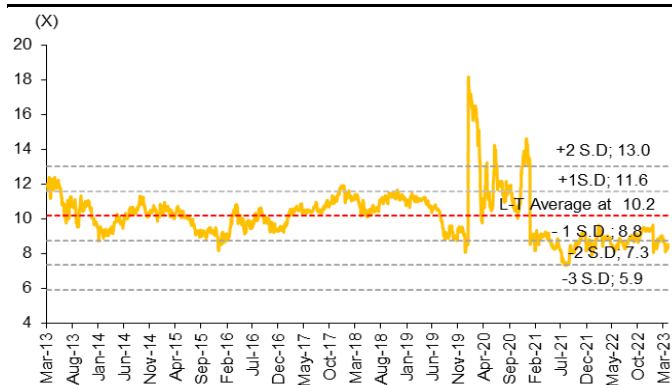
Fig 3: P/E band
