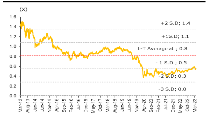
Fig 4: P/BV band
