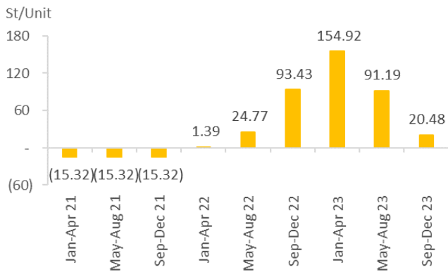
Figure 12: Ft rate
