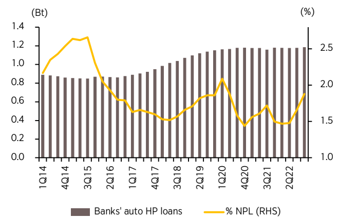
Figure 4: NPL outlook
