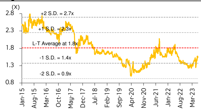
Figure 5: NYT's P/BV band
