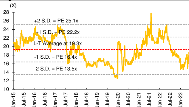
Figure 4: NYT's P/E band
