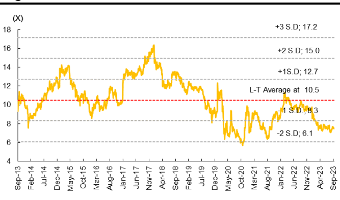
Fig 4: P/E band
