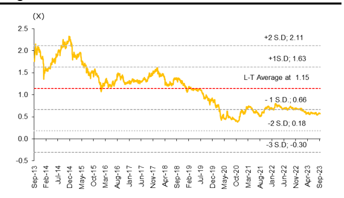
Fig 5: P/BV band
