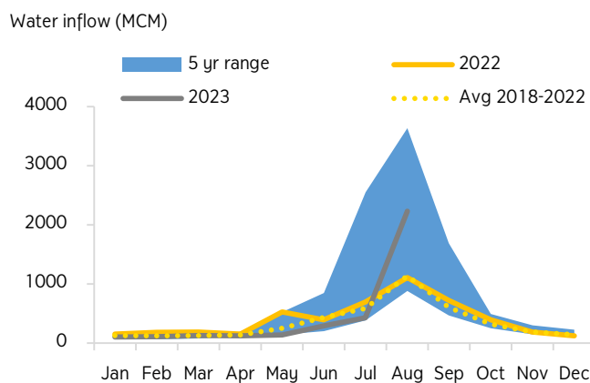
Figure 1: NN2 Water inflow
